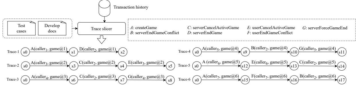
Fig. 1: Six game invocation sequences for GameChannel.
