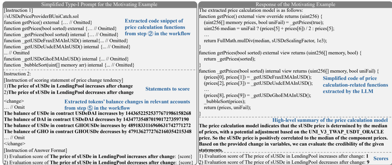
Fig. 3. The simplified Type-I prompt and its response for the motivating example during the inference process.
